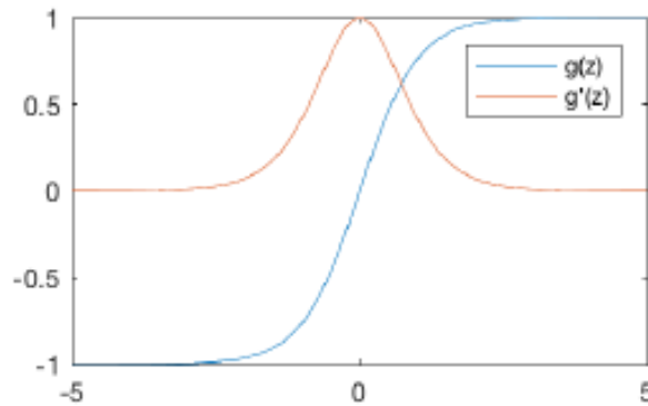
Hyperbolic Tangent
